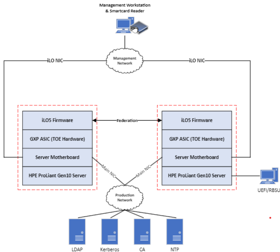
Figure 2: TOE Deployment
